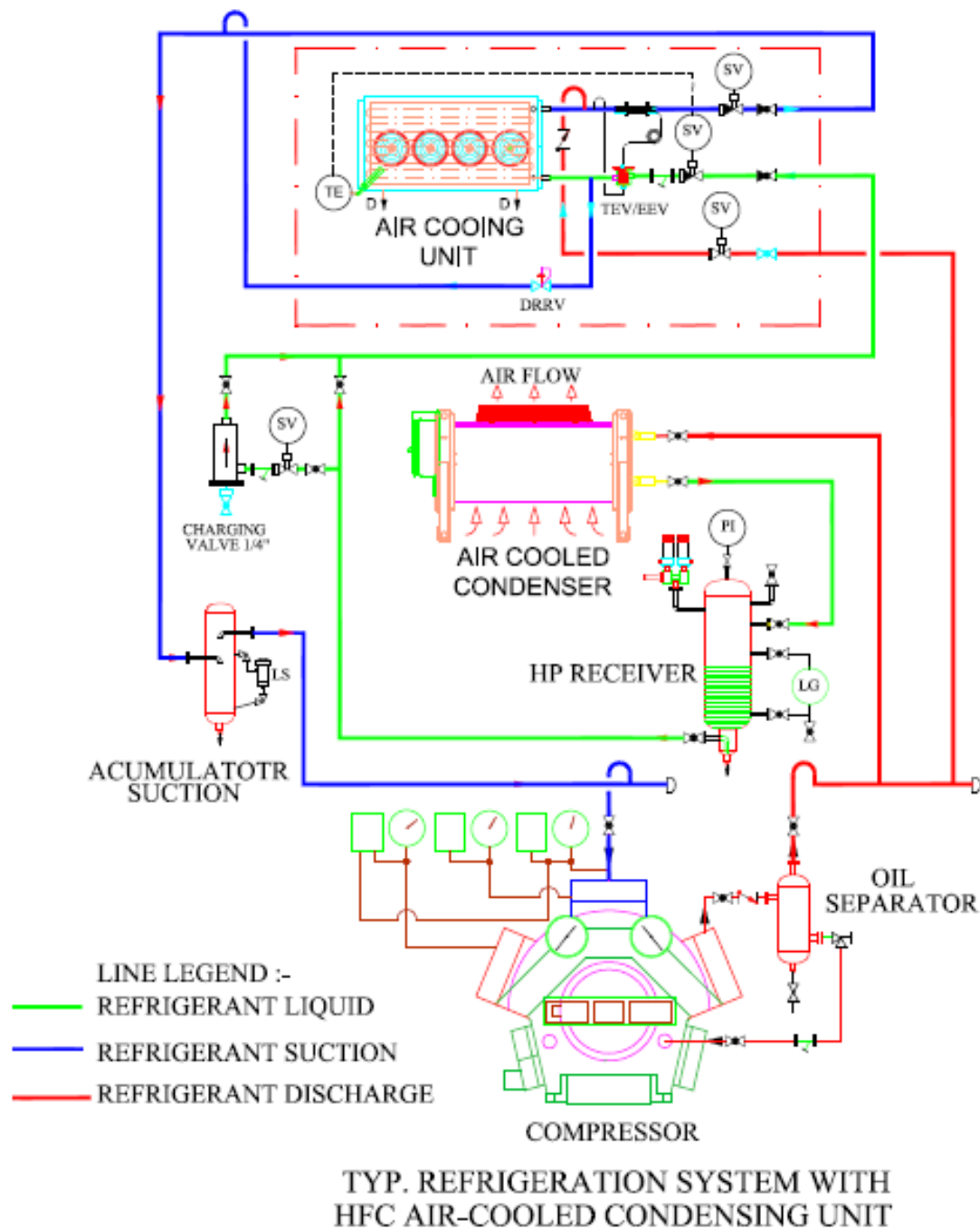
Figure 16: Typical P&ID for Refrigeration Systems
