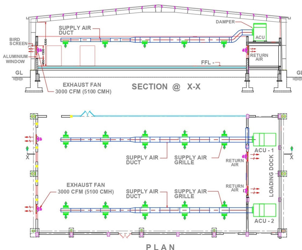
Figure 18: Plan and section showing air-cooling units and distribution for the packing hall.
