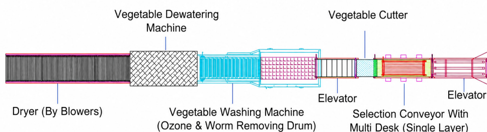
Figure 4: Layout of leafy vegetable line
