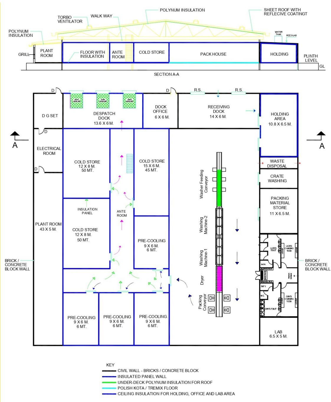
Figure 13: Illustrative layout of a banana packhouse
