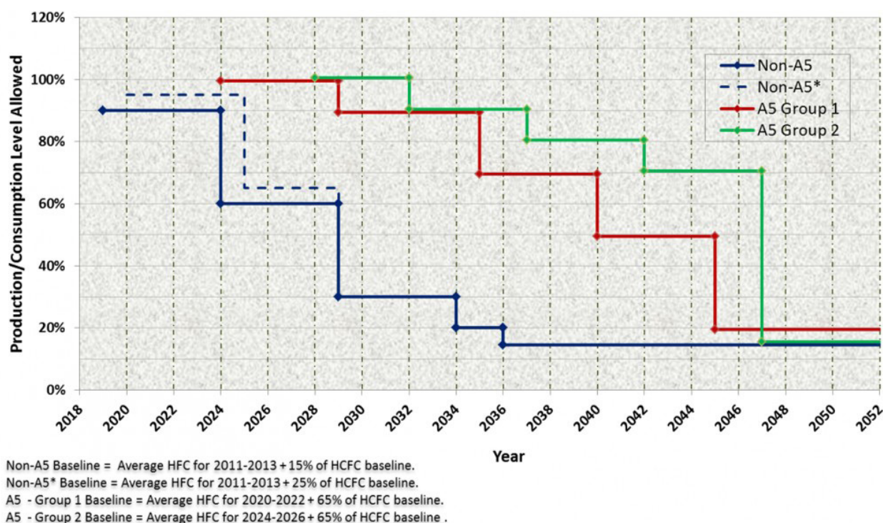
Figure 17: HFCs consumption/production reduction schedule
