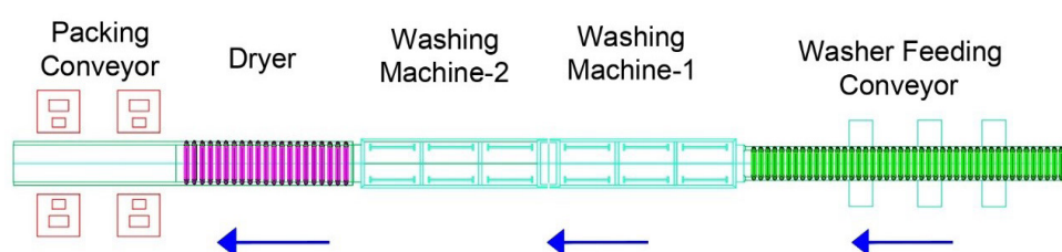
Figure 5: Layout of banana line
