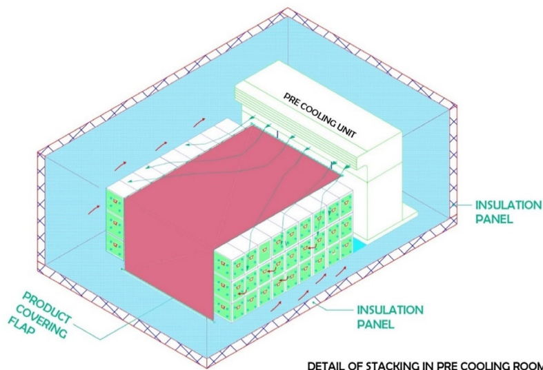
Figure 11: Illustrative diagram for pre-cooling chamber with floor-mounted unit and product stacking
