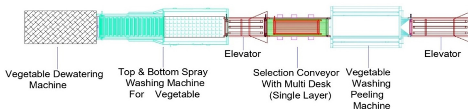
Figure 6: Layout of root vegetable line
