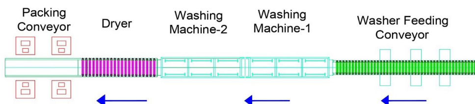
Figure 7: Typical layout of mango line
