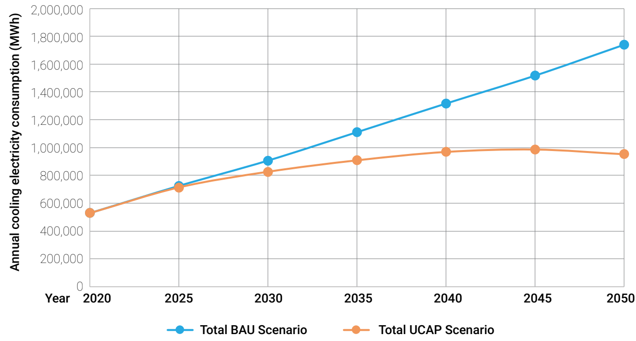
Figure 34: Projections on annual cooling electricity consumptions for specific building types in Can Tho
